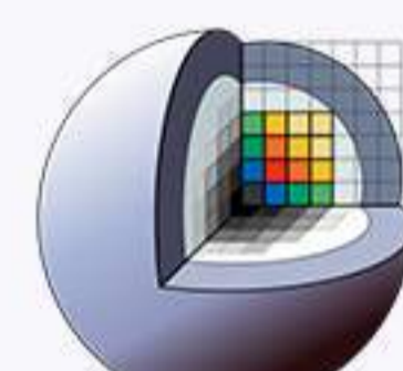
Segmentation-3D Slicer
